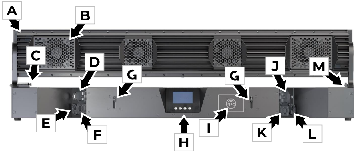
Figure 2. impression X5 Bar IP 1000 overview
