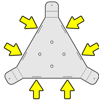
Figure 2. Slots for fixation straps in floor stand
