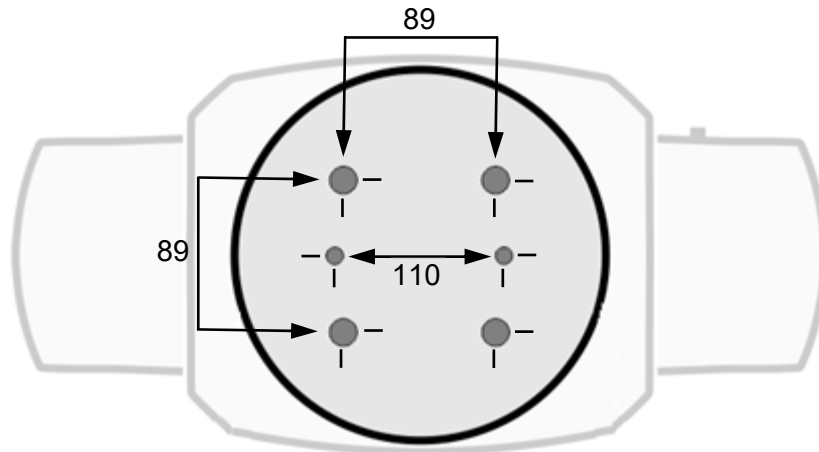
Figure 4. Mounting points in base
