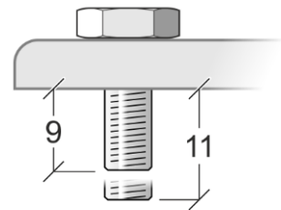
Figure 5. Min./max. bolt protrusion into fixture base (millimeters)
