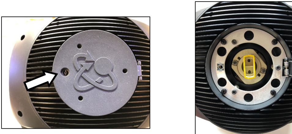
Figure 6. Opening the lamp compartment
